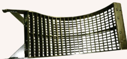
Concavo Axial Central Traseiro - Barra Chata
